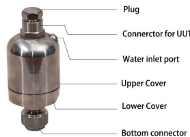
Model 1558 Oil-water isolator, 700 bar, Φ77mm x 155mm, 120ml volume, 0.5mm diaphragm thickness
