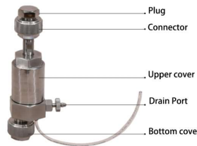
Model 1557 Oil-gas isolator, 700 bar, Φ45mm x 95mm
